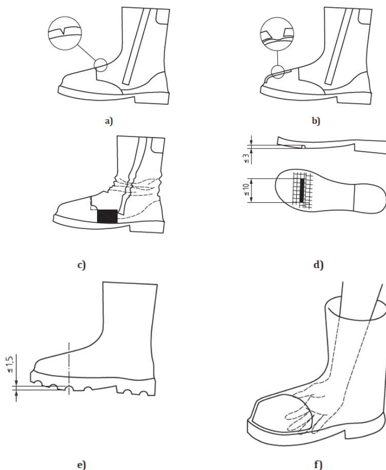
Figure 4 – Damage Assessment guidelines
